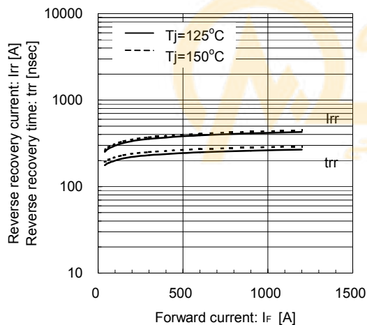
Reverse Recovery Characteristics (typ.) V_{CE}=600V , V_{GE}=\pm 15V , R_g=0.62\Omega , T_J=125^\circ C , 150^\circ C
