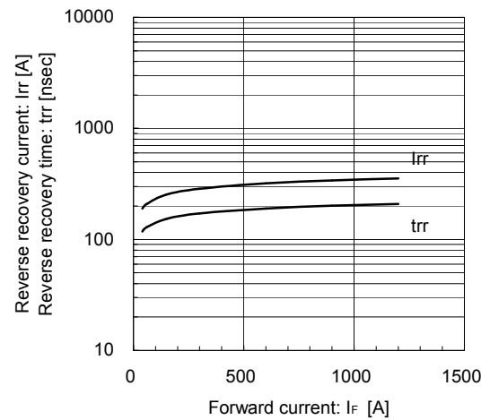
Reverse Recovery Characteristics (typ.) V_{CE}=600V , V_{GE}=\pm 15V , R_g=0.62\Omega , T_J=25^\circ C
