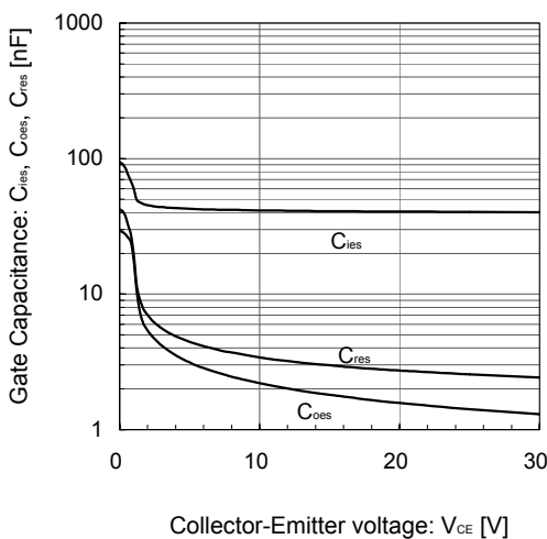
Gate Capacitance vs. Collector-Emittter Voltage (typ.) V GE = 0V, f = 1MHz, T J = 25°C
