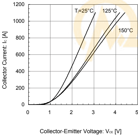
Collector current vs. Collector-Emittter voltage (typ.) V GE = 15V / chip
