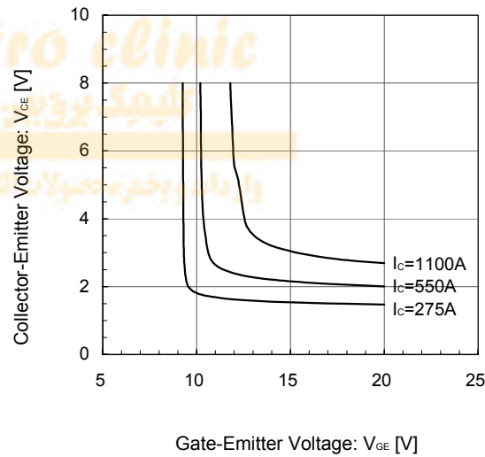
Collector-Emittter voltage vs. Gate-Emittter voltage (typ.) T J = 25°C / chip
