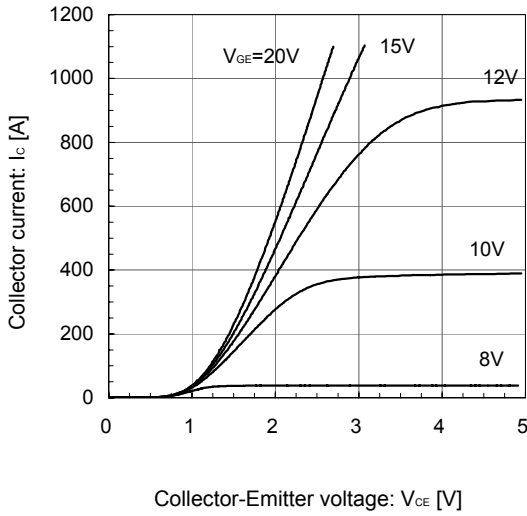
Collector current vs. Collector-Emittter voltage (typ.) T J = 25°C / chip
