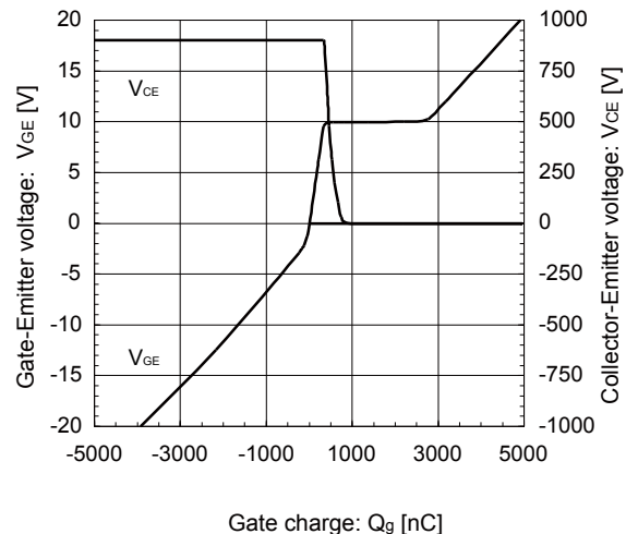
Dynamic Gate Charge (typ.) V CC = 900V, Ic = 550A, T J = 25°C
